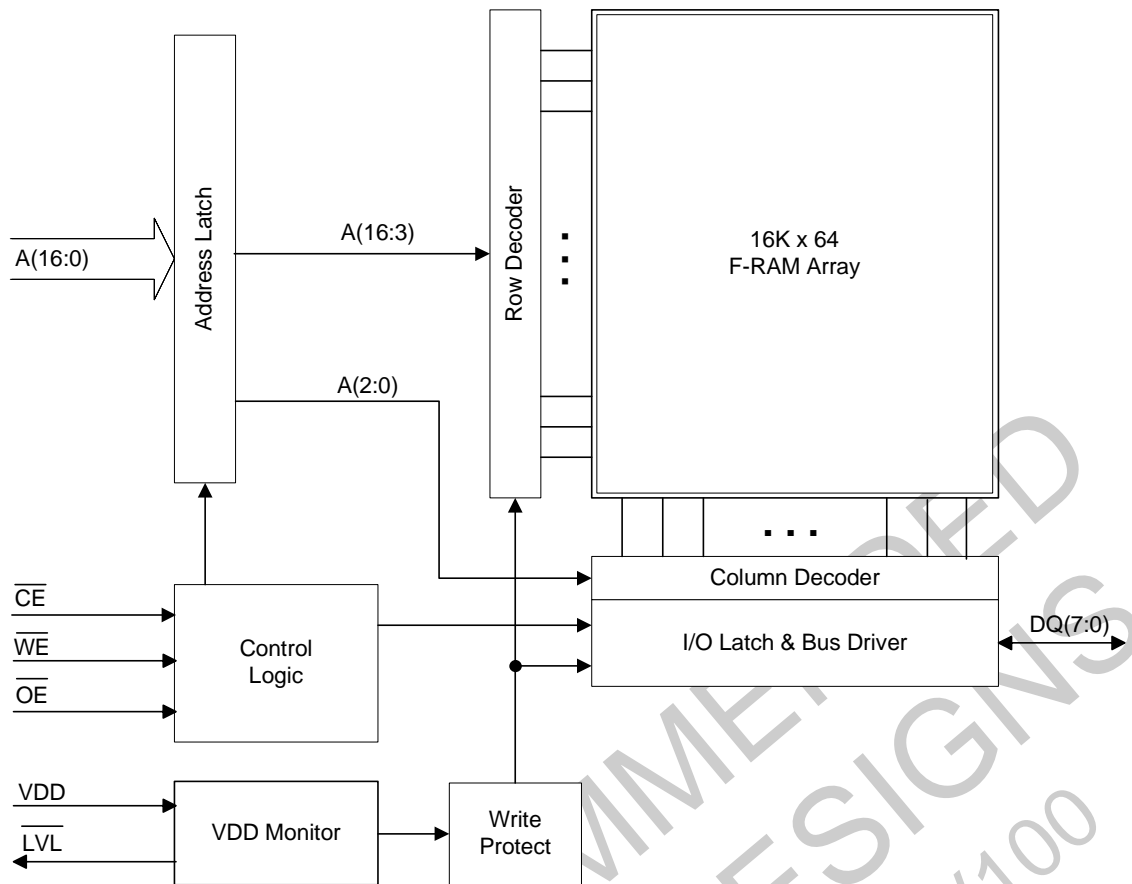
Figure 1. Block Diagram
