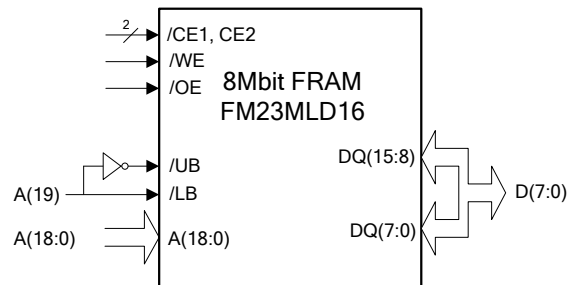
Figure 4. FM23MLD16 Wired as 1Mx8
