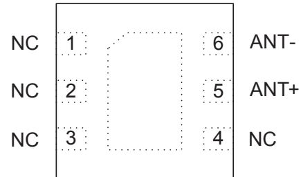
Figure 2: UDFN 6-pin package (top view, PCB layout)
